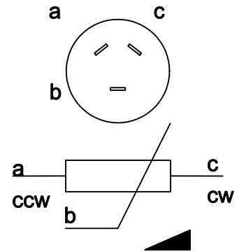
Connection diagram
