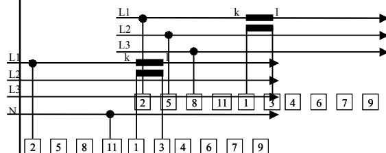
Three-conductor three-phase, asymmetric load 2p3
