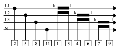
Four-conductor three-phase, asymmetric load 3p4
