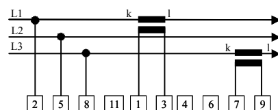
Three-conductor three-phase, asymmetric load 2p3
