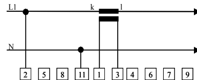
Single-phase AC 1p2
